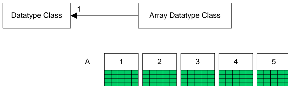
Figure 4: In an HDF5 dataset with an array datatype, each data element is itself an array.
