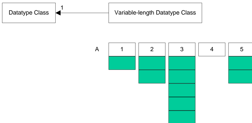
Figure 3: Each data element of a dataset with a variable-length datatype can be of a different size.
