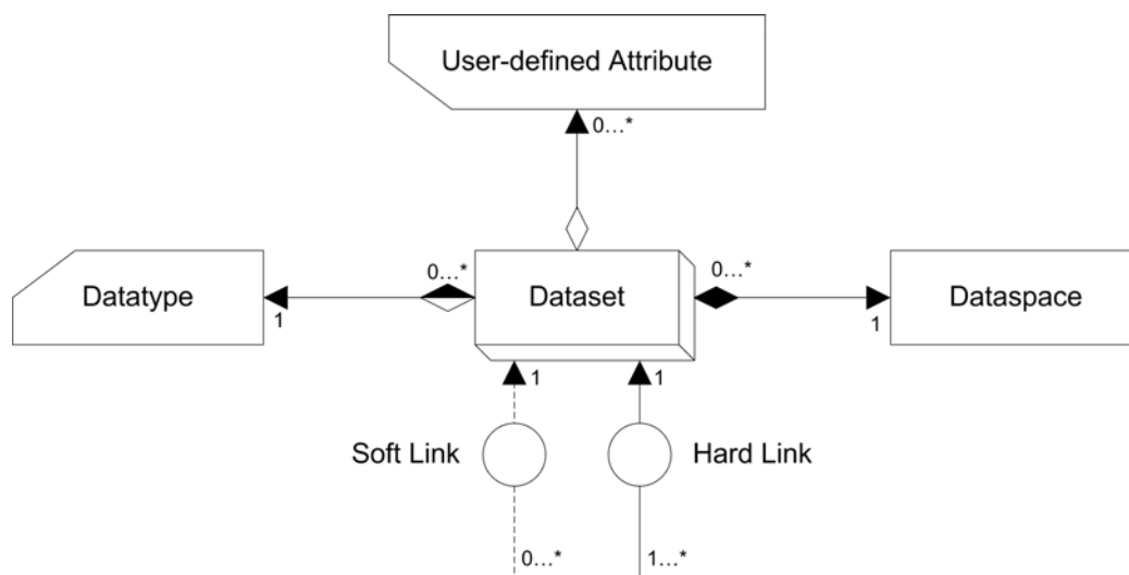
Figure 5: A dataset has a datatype, a dataspace, and optional attributes, and can be linked into the file hierarchy with both soft and hard links.
