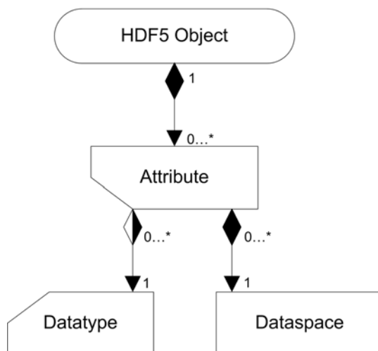
Figure 6: An attribute is attached to an HDF5 object.
