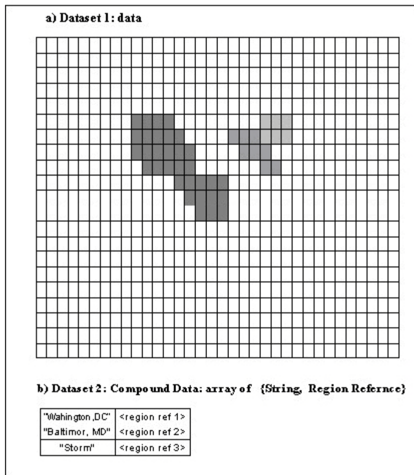
Figure 7-14. Storing the table with a compound datatype
