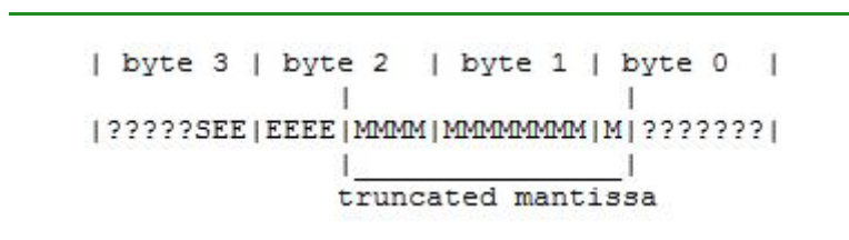
Figure 5-16. Passed to the n-bit filter
