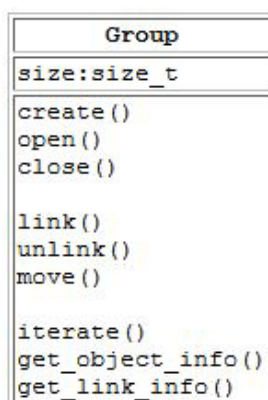
Figure 4-6. The group object
