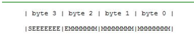
Figure 5-15. H5T_NATIVE_FLOAT in memory
